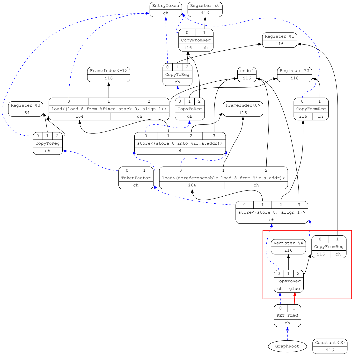
dag-combine1 input for getAValentry
