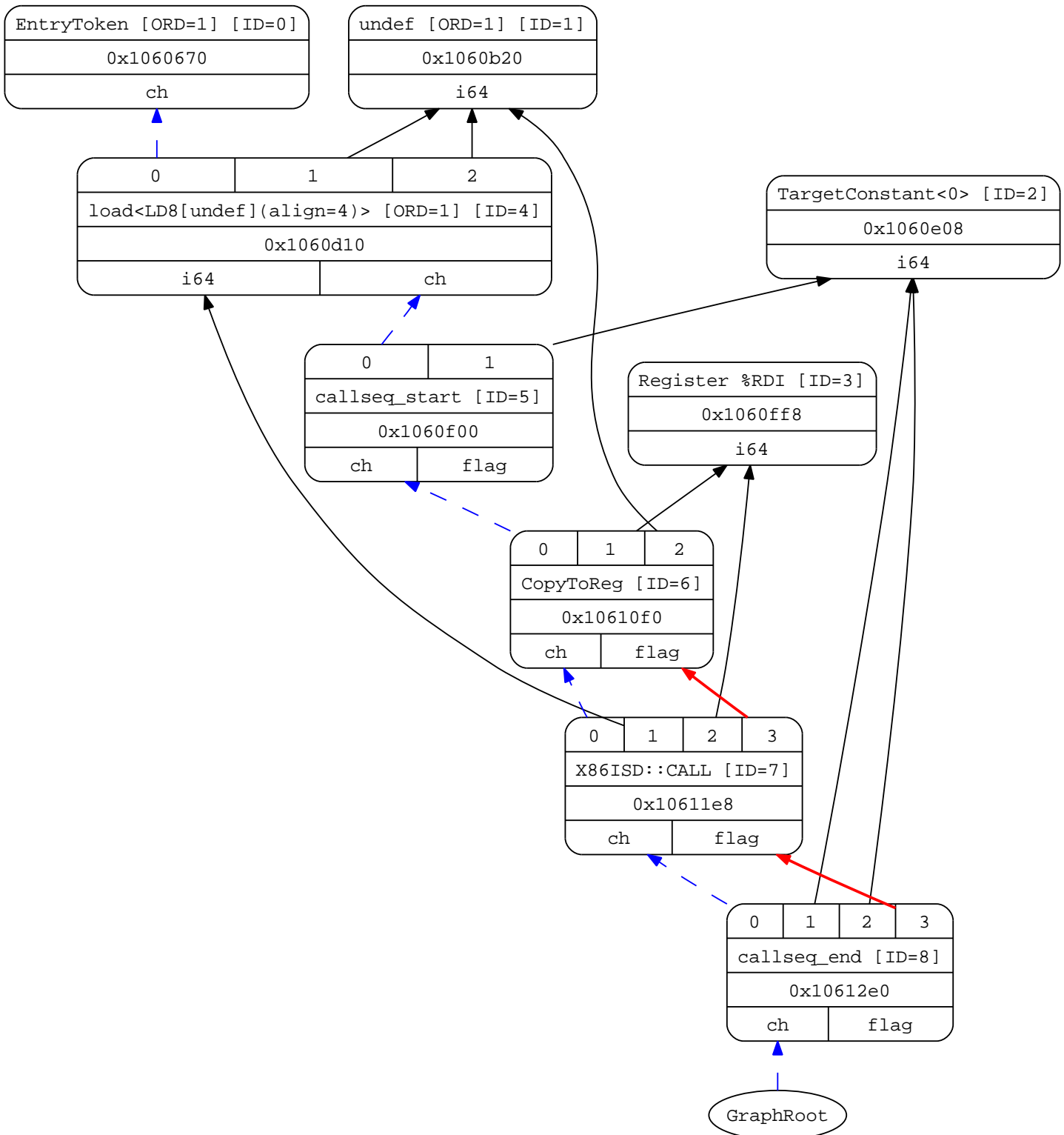
isel input for ArgsFree:entry
